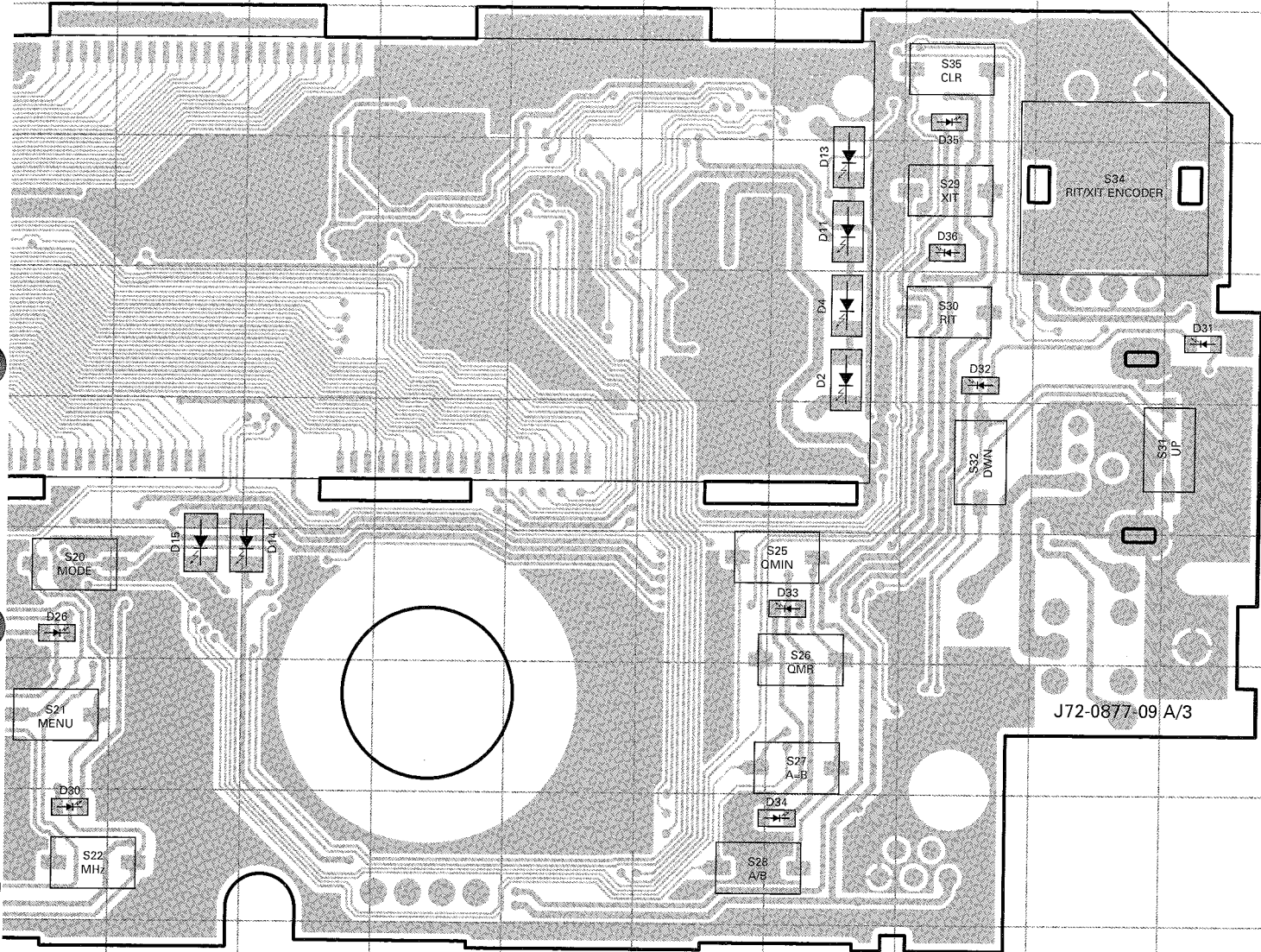
DISPLAY UNIT (X54-3410-00) (A/3, B/3, C/3) Component side view (J72-0877-09)
