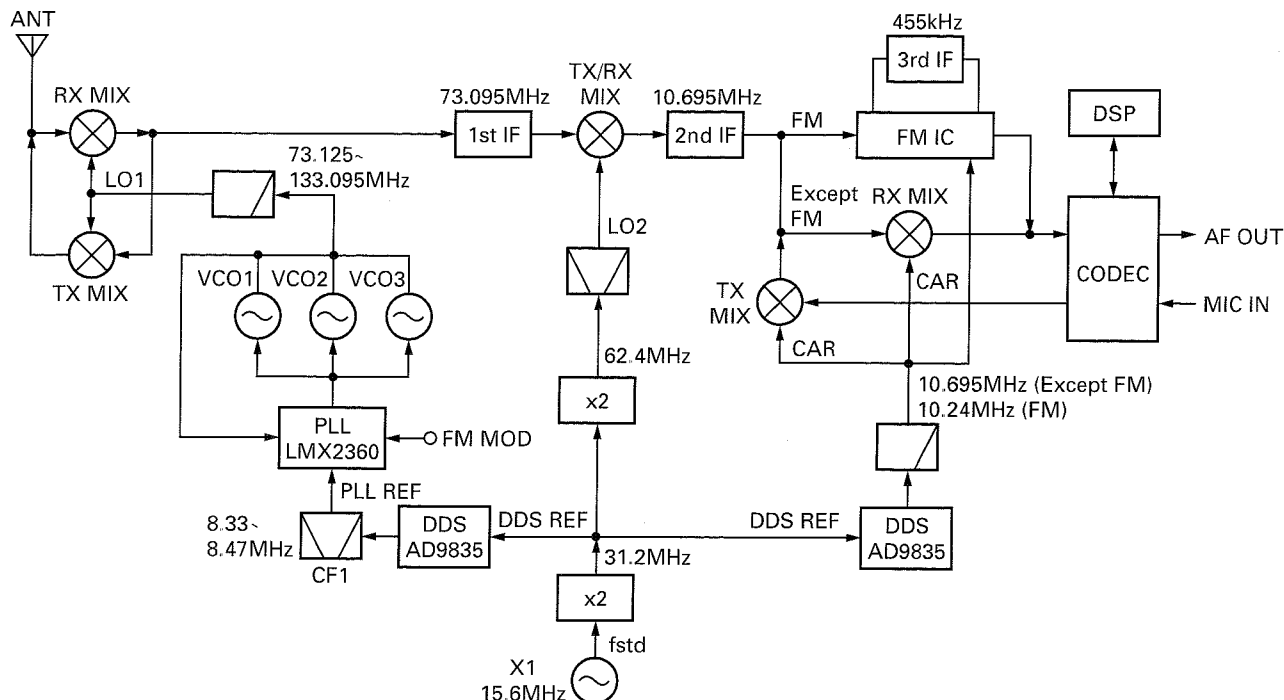
Fig. 1 Frequency configuration
