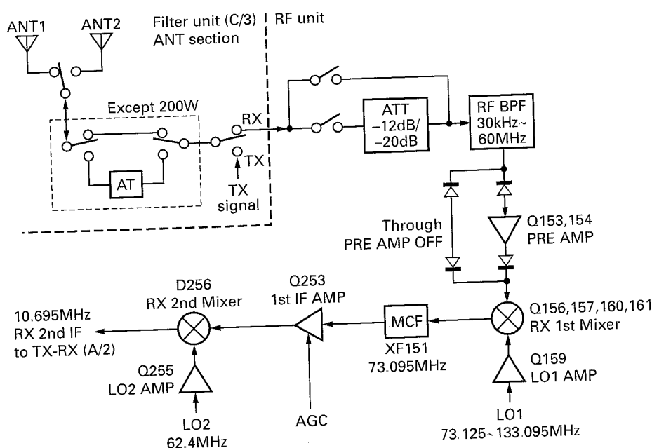
Fig. 3 From antenna to the second IF frequency (10.695MHz)
